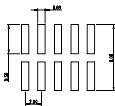
Recommended P.C.B Layout(±0.05)
